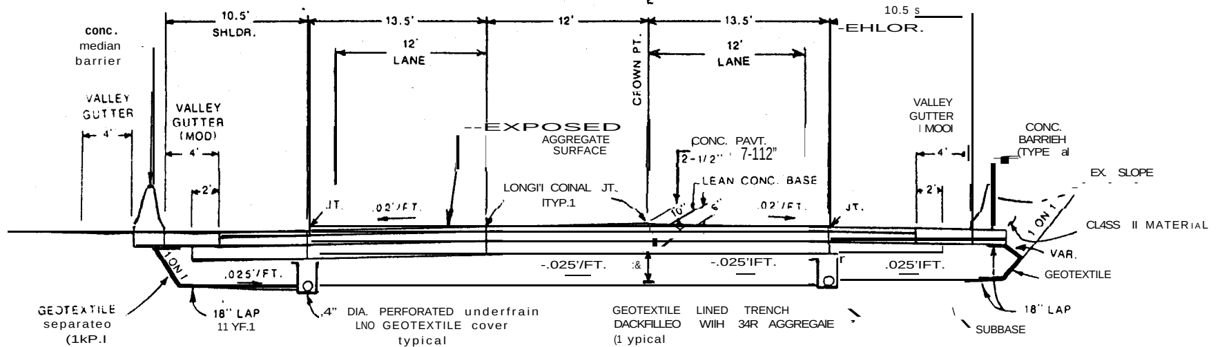
figure 1. Typical cross-sections trial project.
