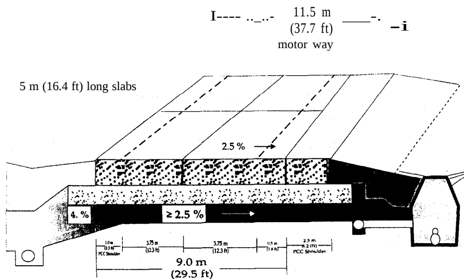
Figure 2. German concrete pavement geometric elements.
