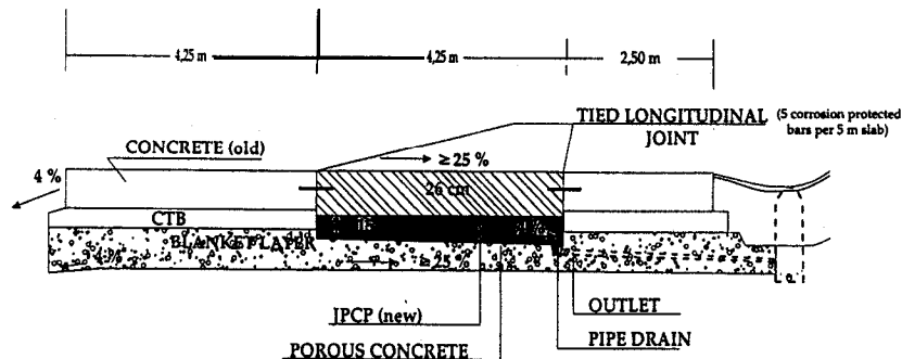
Figure 4. Designs for renewal of old concrete pavements in Germany.
